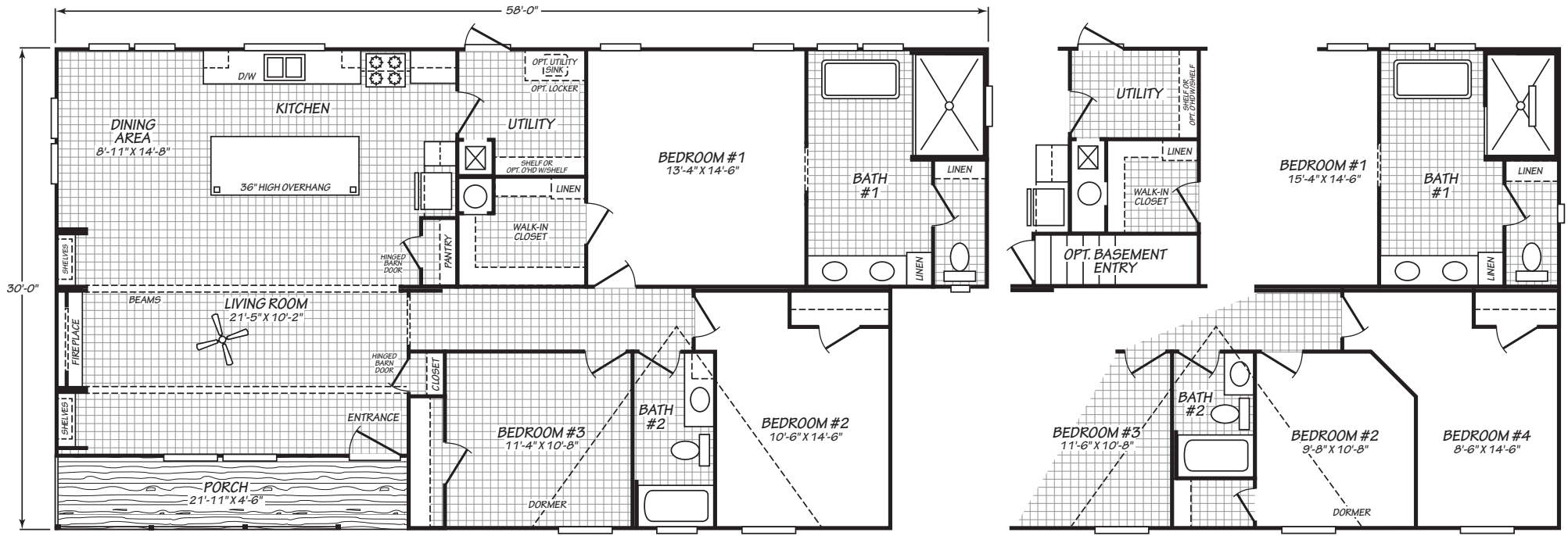
OPT. BEDROOM #4 (WITH 2' STRETCH)
